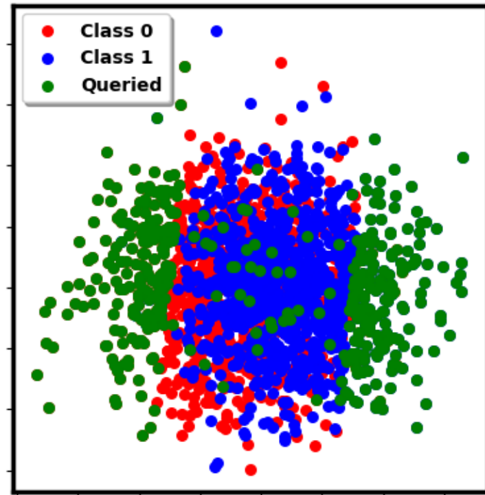
Bimodal Querying: Amplifying Distributional Separation
